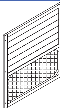
6 MAIN COOP BACK PANEL X 1PC
