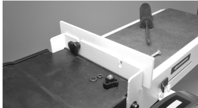
Figure 3 - Install fence knobs.
