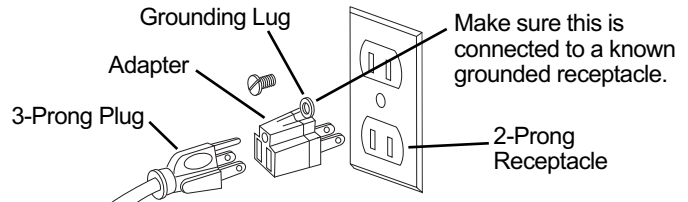
Figure 13 – 2-Prong receptacle with adapter
