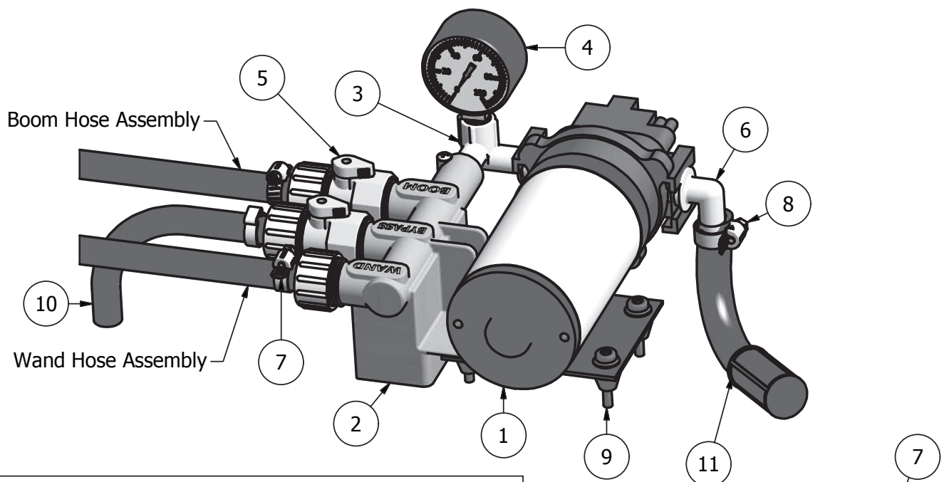
PARTS LIST
