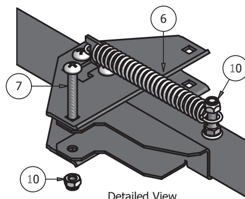
Detailed View
