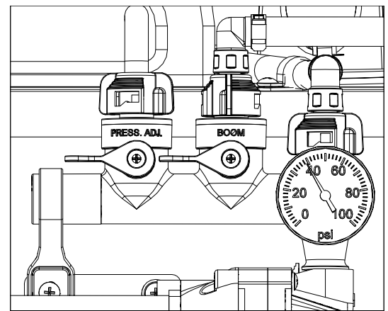
Manifold Valves CLOSED
