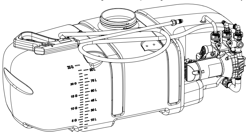
Tank/Plumbing Pre-Assembly
