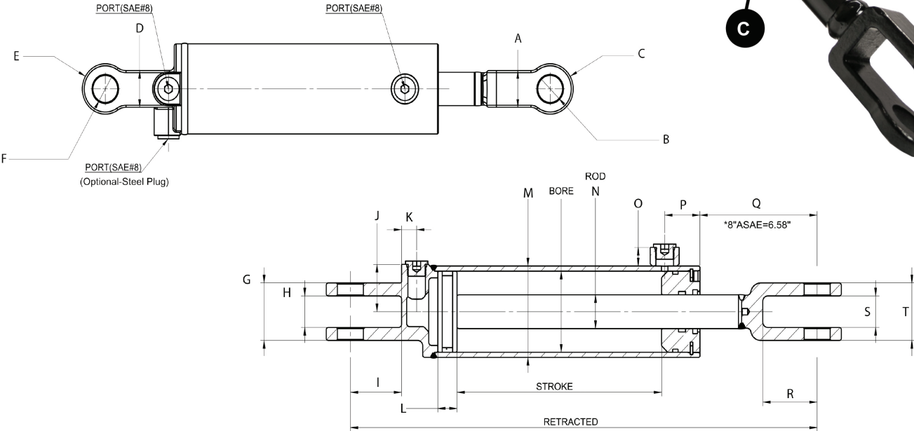
DIMENSIONAL DATA IN INCHES ( FOLLOWED BY MM)
