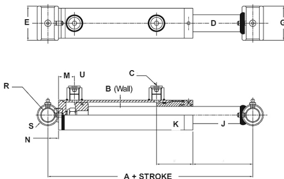
Dimensional Data in Inches (Millimeters)
