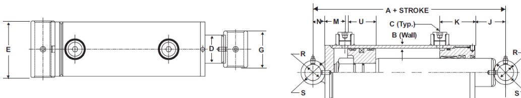
Dimensional Data in Inches (Millimeters)
