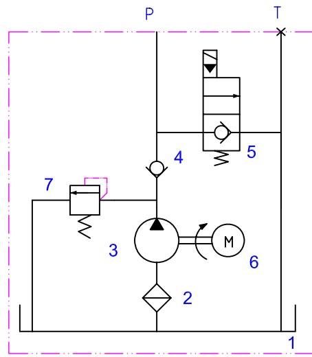
Hydraulic Schematic
