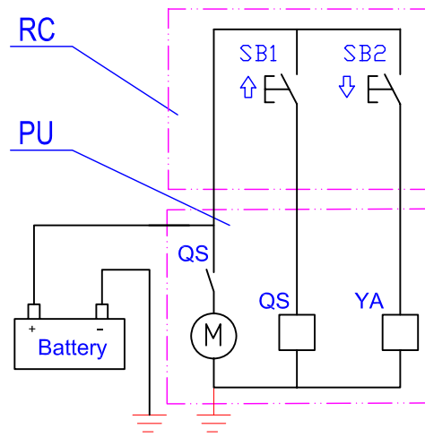
Electric Schematic
