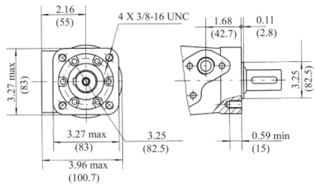
H4 - SAE -"A" 4 BOLT
