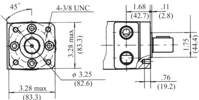
H4 - SAE -"A" 4 BOLT
