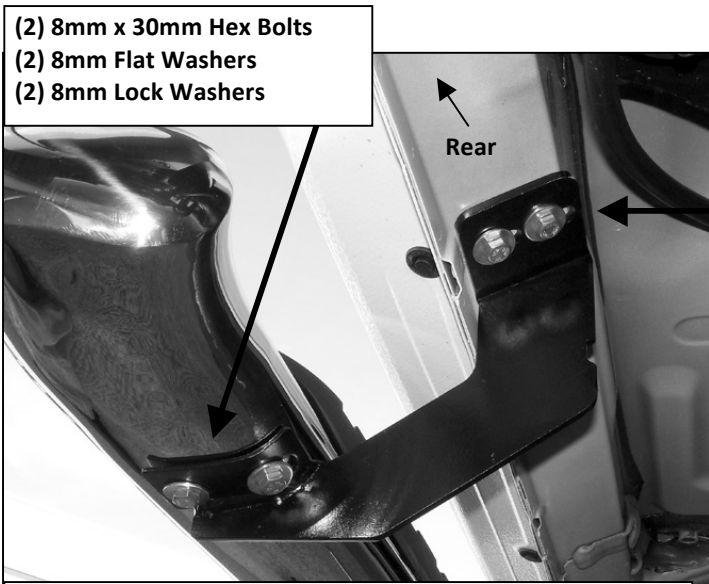
(Fig 3) Driver side rear mounting location pictured
