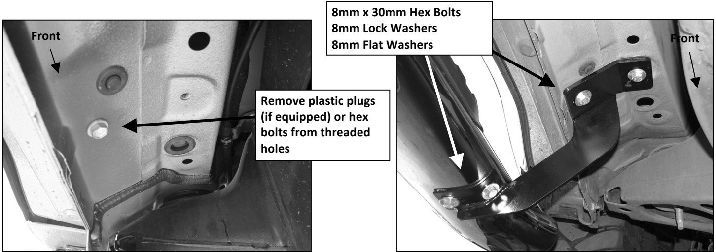
(Fig 1) Driver/Left Front Mounting Location Pictured
