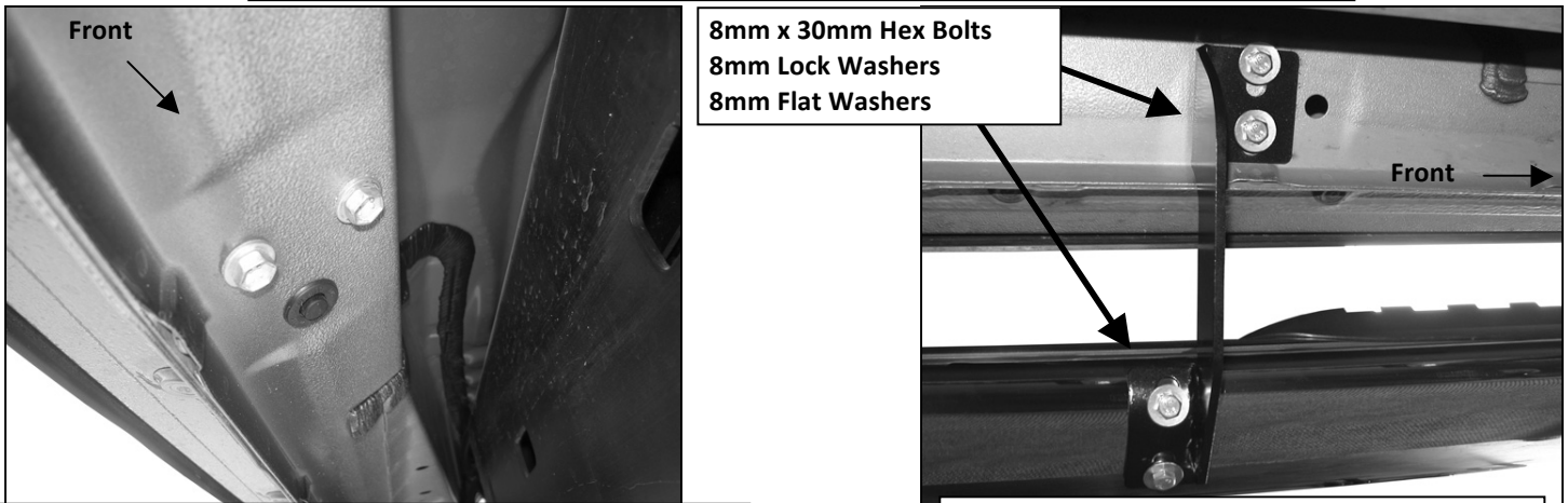
(Fig 4) Driver/Left Center Bracket Pictured
