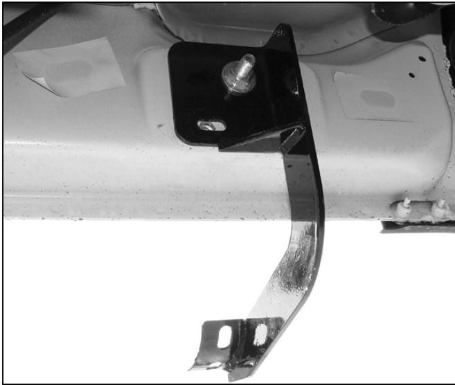
(Fig 3A) Driver/Left front Mounting Bracket
