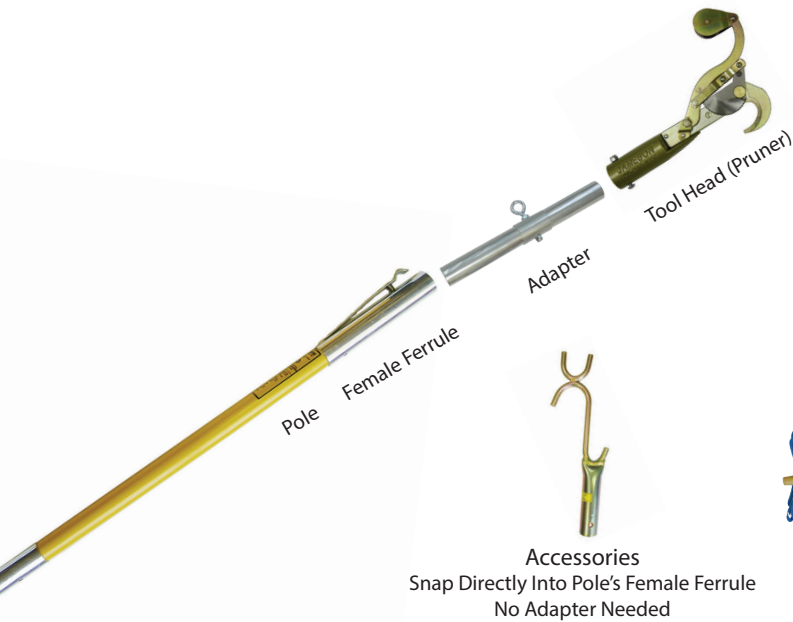
Pruners With Adapters Snap Into Pole's Female Ferrule
