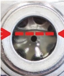
Figure 5 – Vacuum Pump Sight Glass Fill oil above the small circle in the center.
