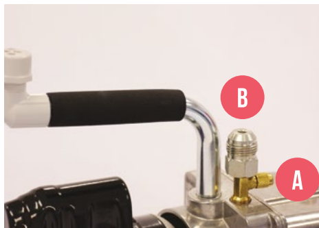
Figure 1 - Vacuum Pump Connections (A) Hand tighten vacuum hose (B) Connect large clear tube, tighten with crescent wrench.
