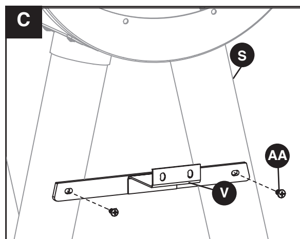
DGSS675CB-D support de raccordement
