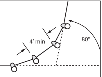
Illustration 8-4 CORNER - FOUR POST Commonly used at the intersection of two roads.
