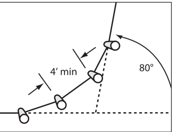
Illustration 8-4 CORNER - FOUR POST Commonly used at the intersection of two roads.
