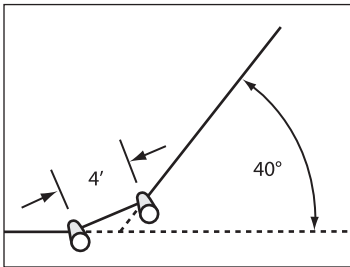
Illustration 8-2 CORNER - DOUBLE POST
