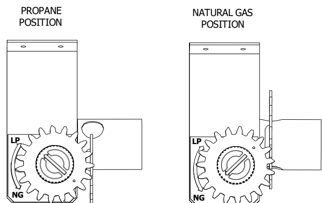
Fig. 8 - Selector Valve
