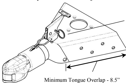
Minimum Tongue Overlap - 8.5"
