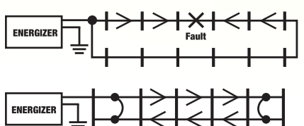
EXAMPLE C - FENCE LOOPS BACK TO ENERGIZER
