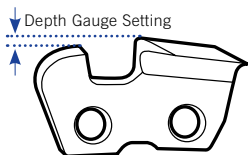
CORRECT DEPTH GAUGE
