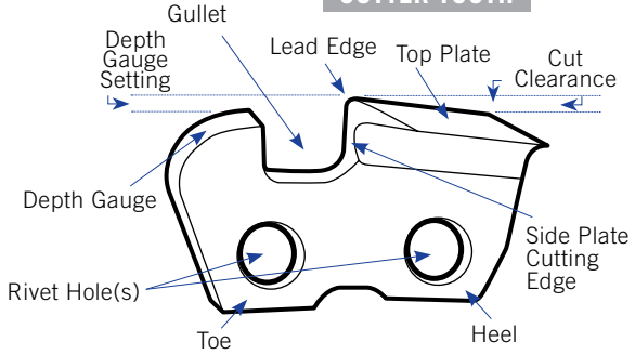
CUTTER TOOTH
