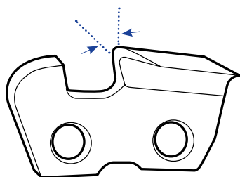
HOOKED CUTTER
