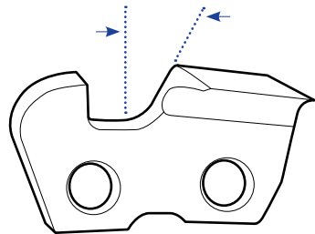
BACKSLOPE CUTTER
