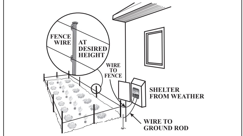
Diagram 5. Fence Installation
