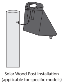
Solar T-Post Installation (applicable for specific models)
